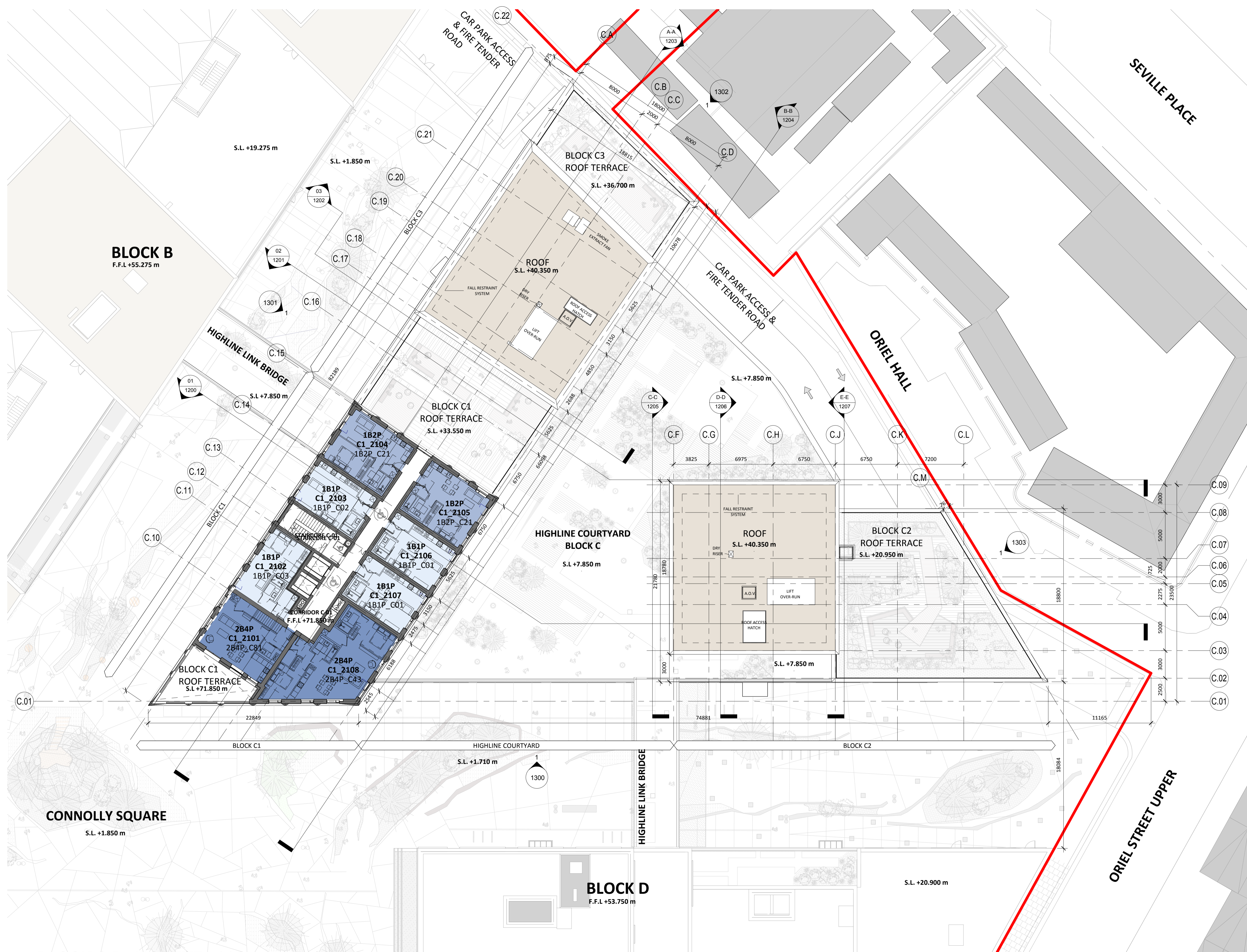
1 BLOCK C PLAN_LEVEL 21 1 : 200
